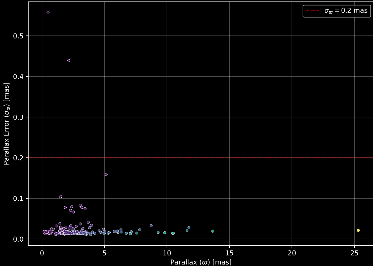
APOGEE DR17 Field: [JHelum1] Parallax Quality (n= 179)
