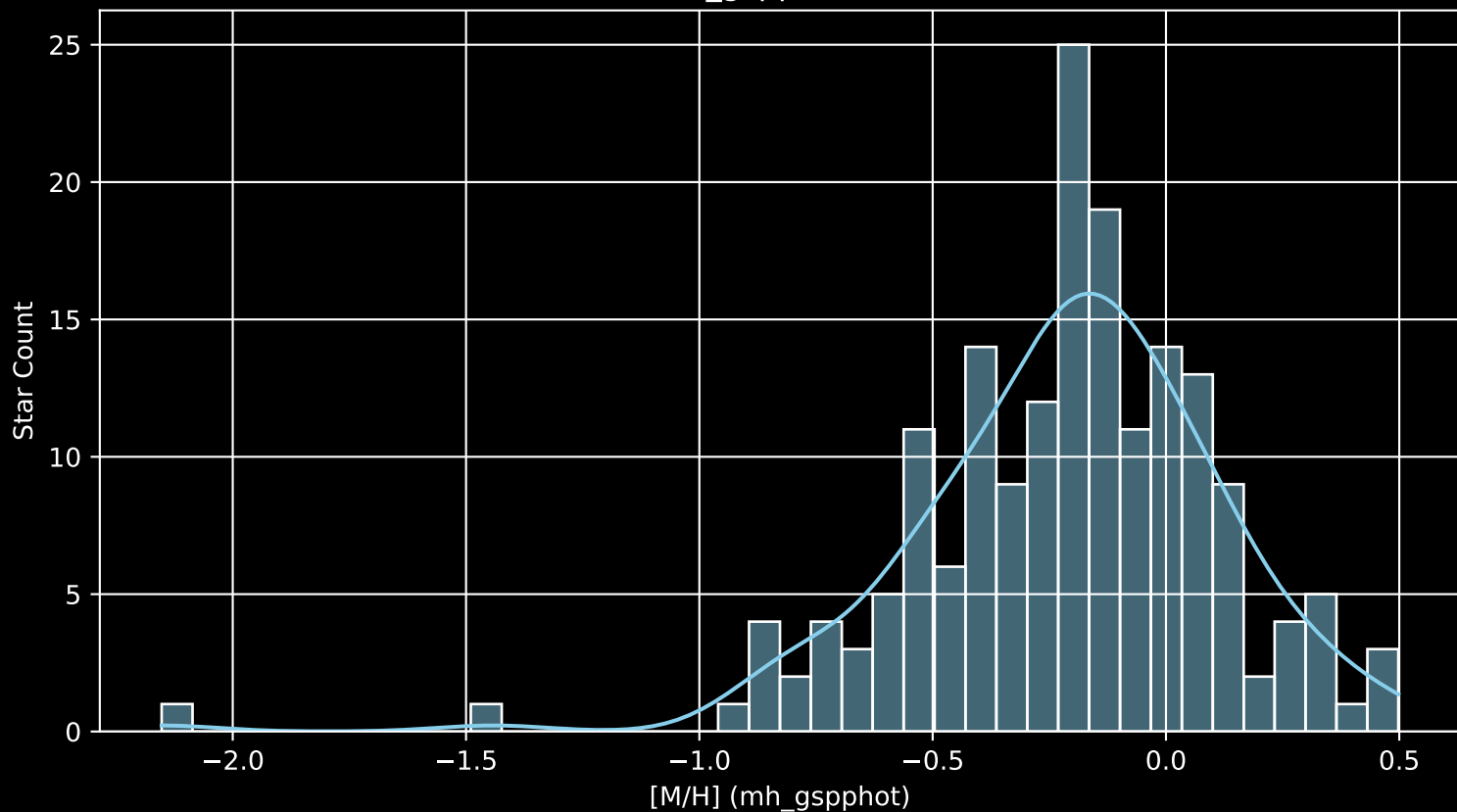
APOGEE DR17 Field: [JHelum1 [M/H] (mh_gspphot) (n= 179)
