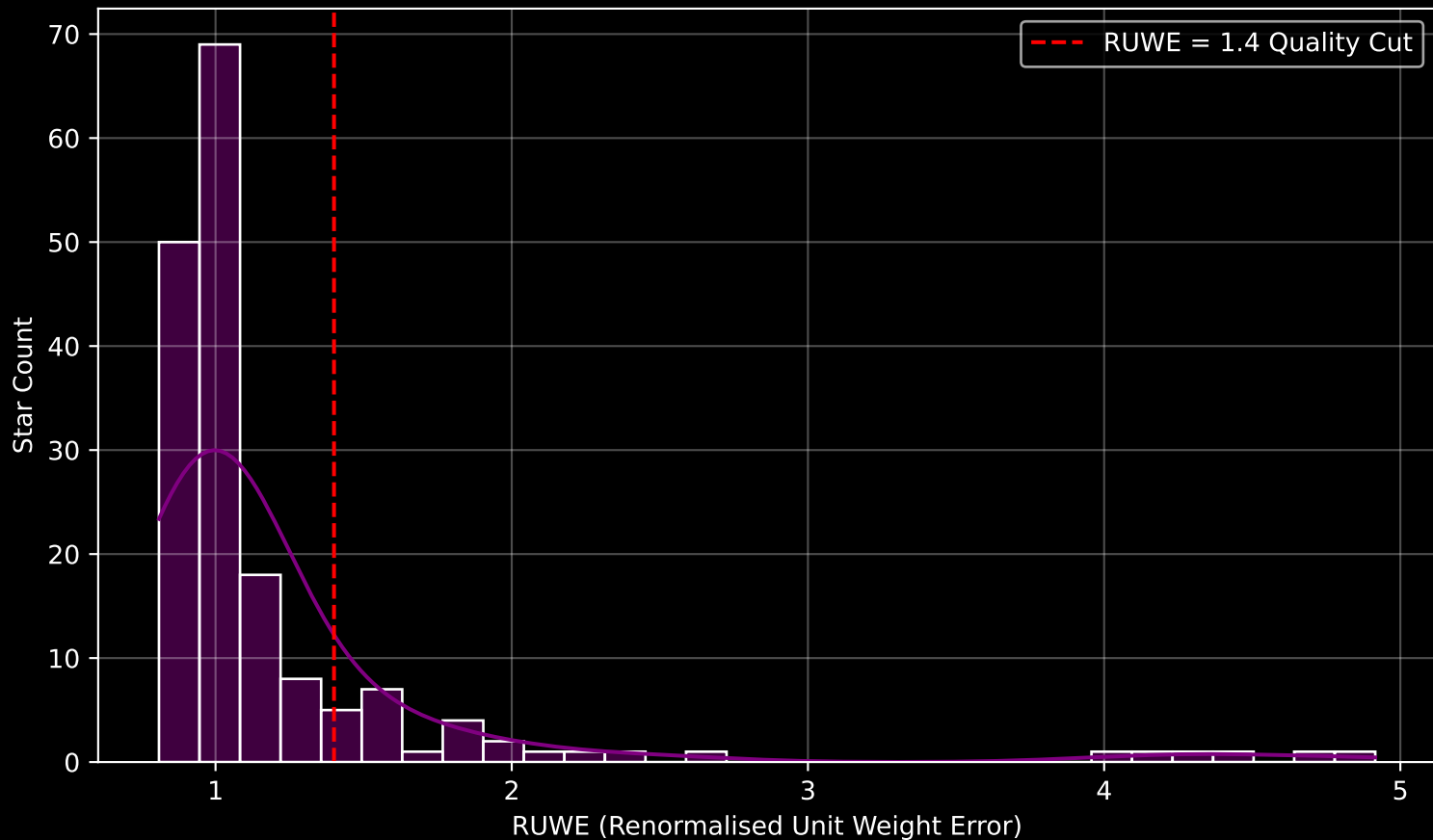
GAPOGEE DR17 Field [JHelium1] RUWE Distribution (n= 174)
