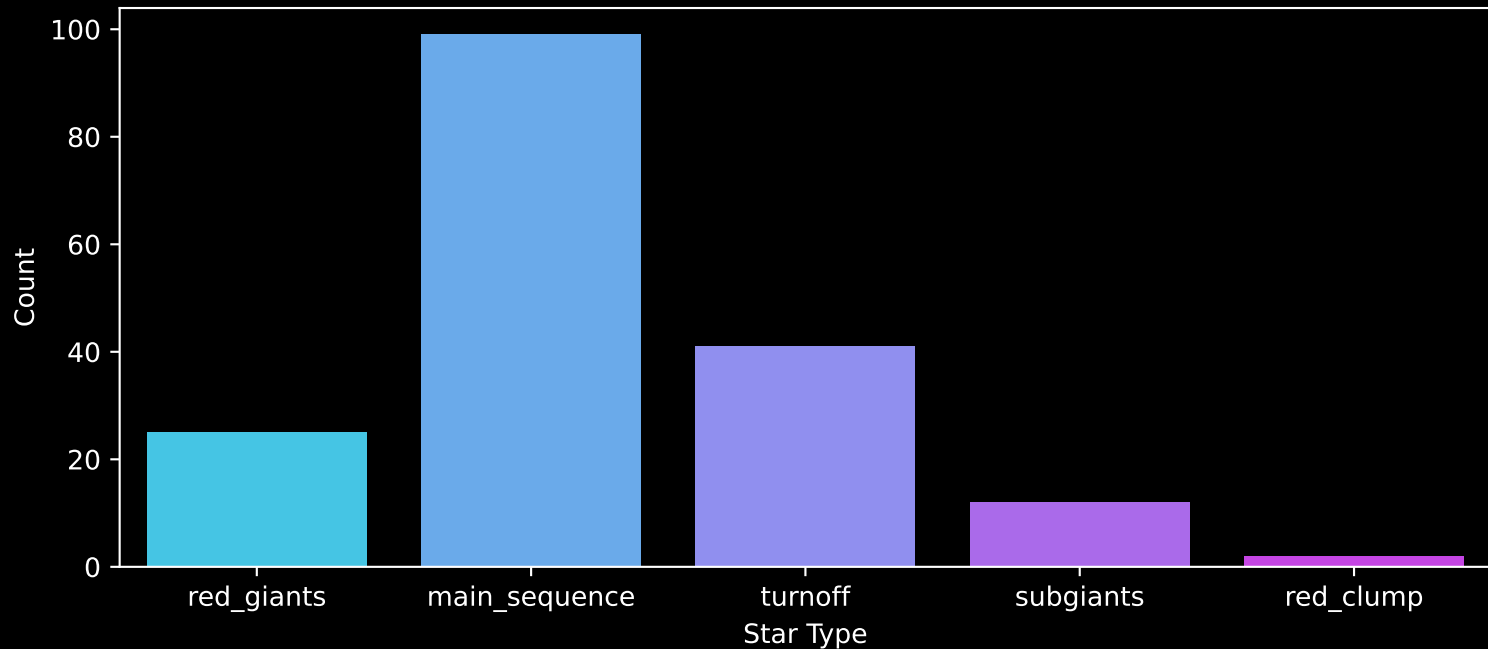
APOGEE DR17 Field: [JHelum1] Count plot of Star Type
