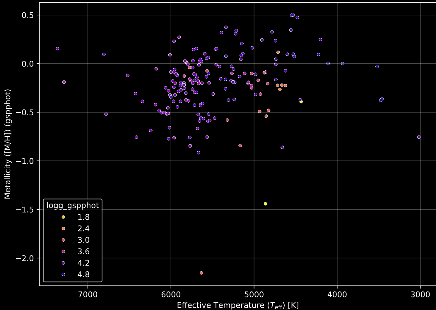
APOGEE DR17 Field: [JHelium1] Stellar Population Parameters (n= 179)
