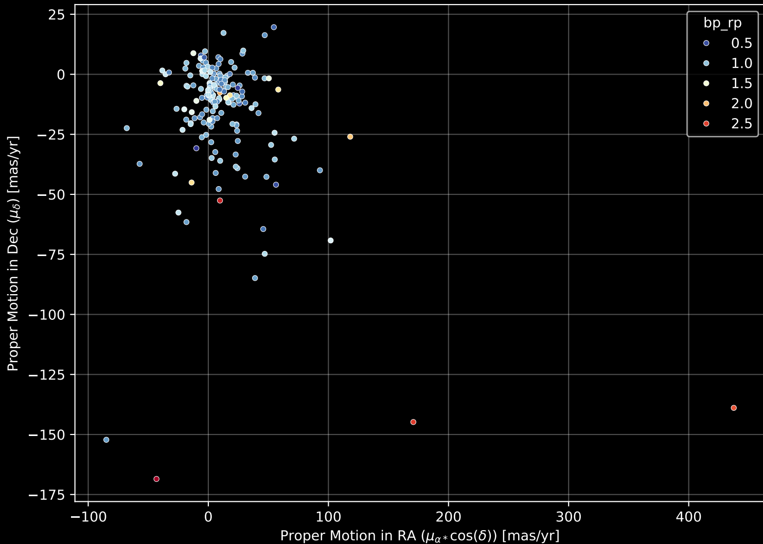
APOGEE DR17 Field: [JHelum1] Proper Motion Diagram (n= 179)
