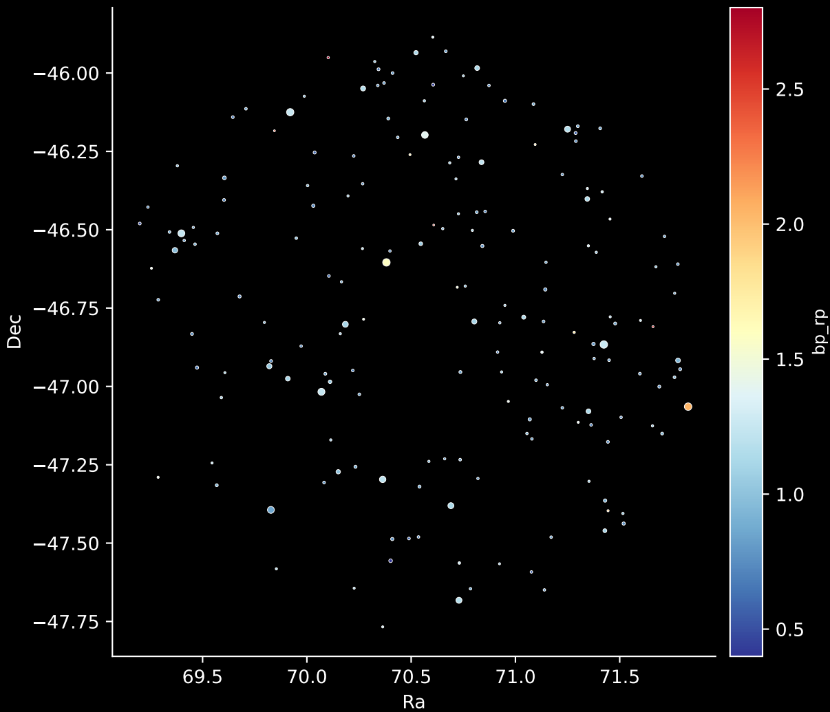
APOGEE DR17 Field: [JHelum1] Stars: 179
